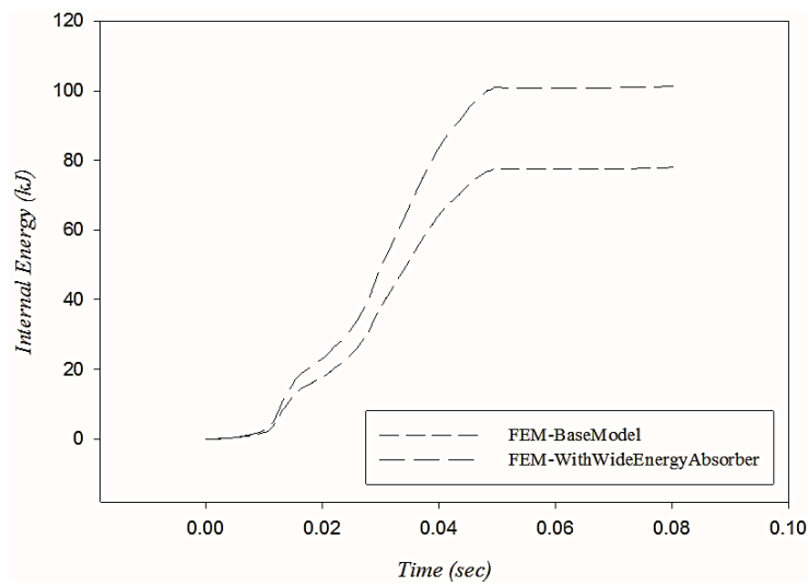
Fig19. Time histories of the internal energy for designs with and without the tapered wide multi-cell energy absorber.
